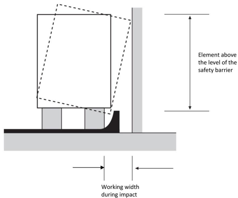
Figure 15 Working Width For Concrete Barriers
