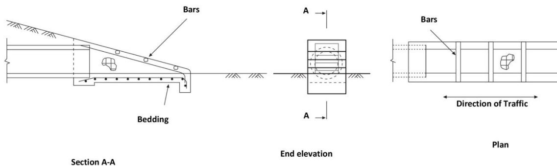
Drivable Culvert End Wall for a Small Pipe
