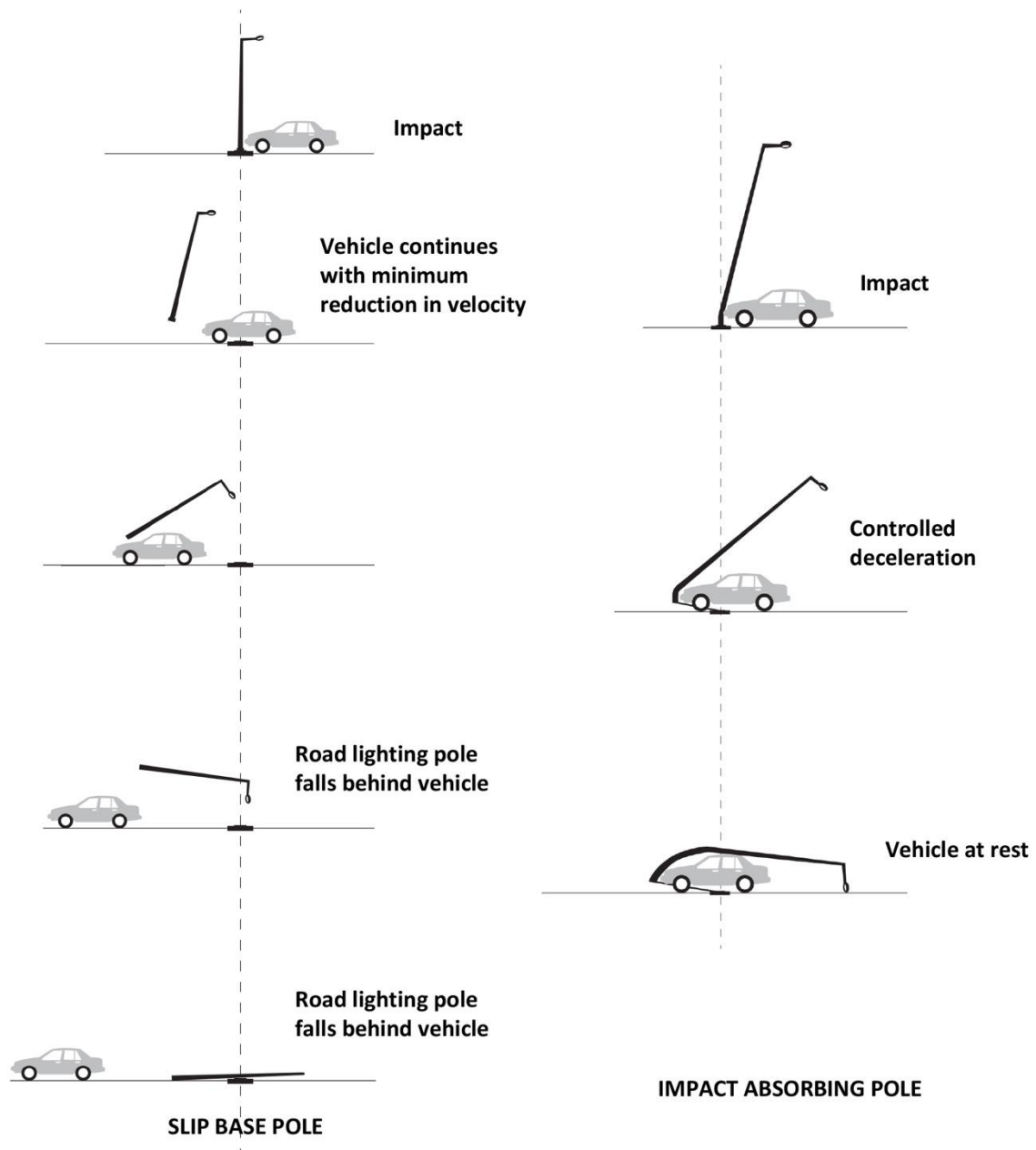
Figure 16 Operation of Frangible Lighting Columns
