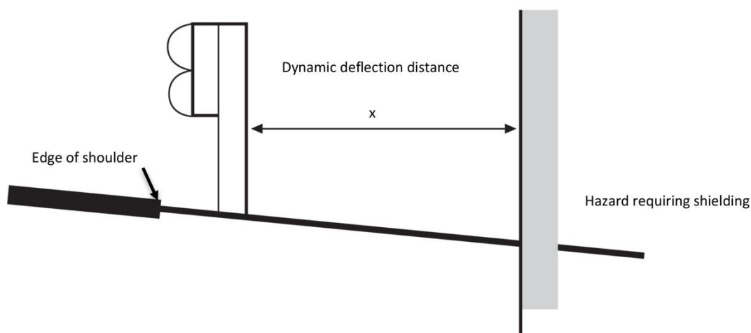
Figure 8 Deflection Clearance Required Between Barrier and Hazard
