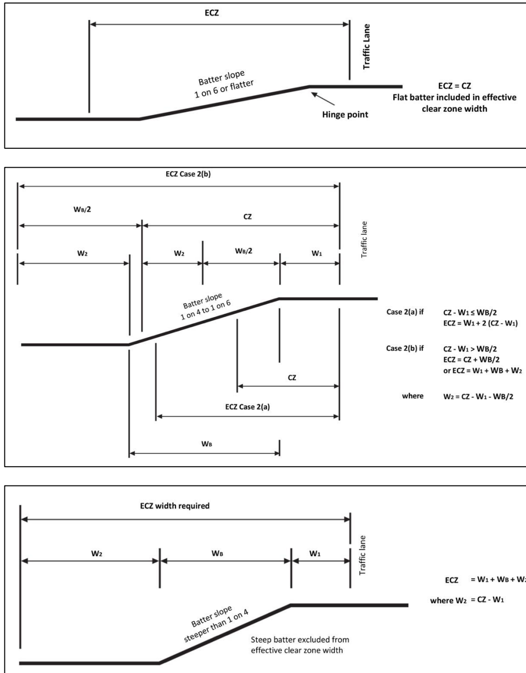
Figure 3 The Effect Of Side Slopes On Clear Zones Widths
