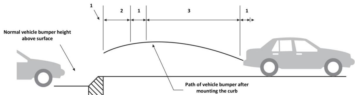
Figure 11 The Effect of Curb on the Trajectory of an Impacting Vehicle
