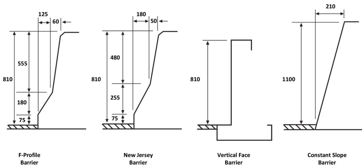
Figure 7 Four Common Rigid Barrier Profiles
