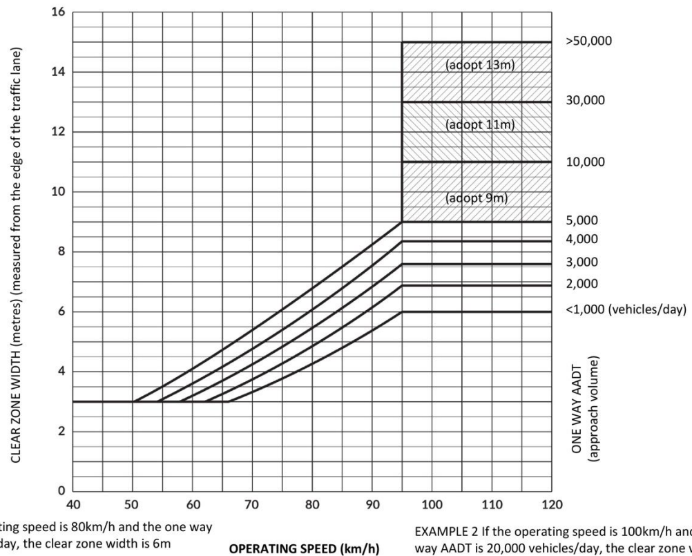
Figure 1 Clear Zone for Straight Roads
