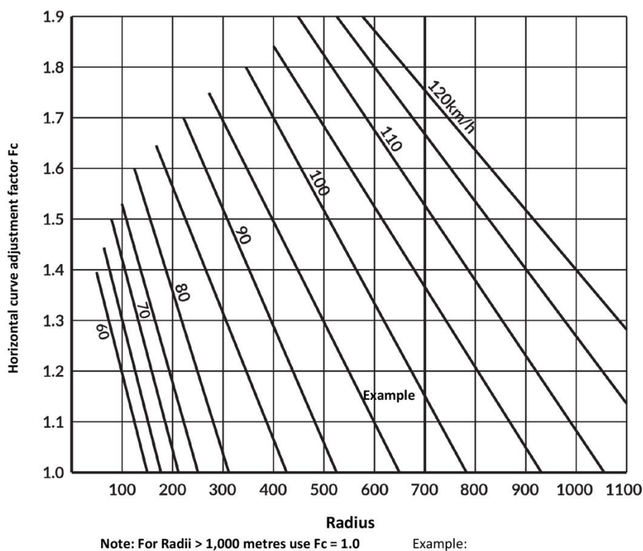
Figure 2 Clear Zone Adjustment Factors for Curves
