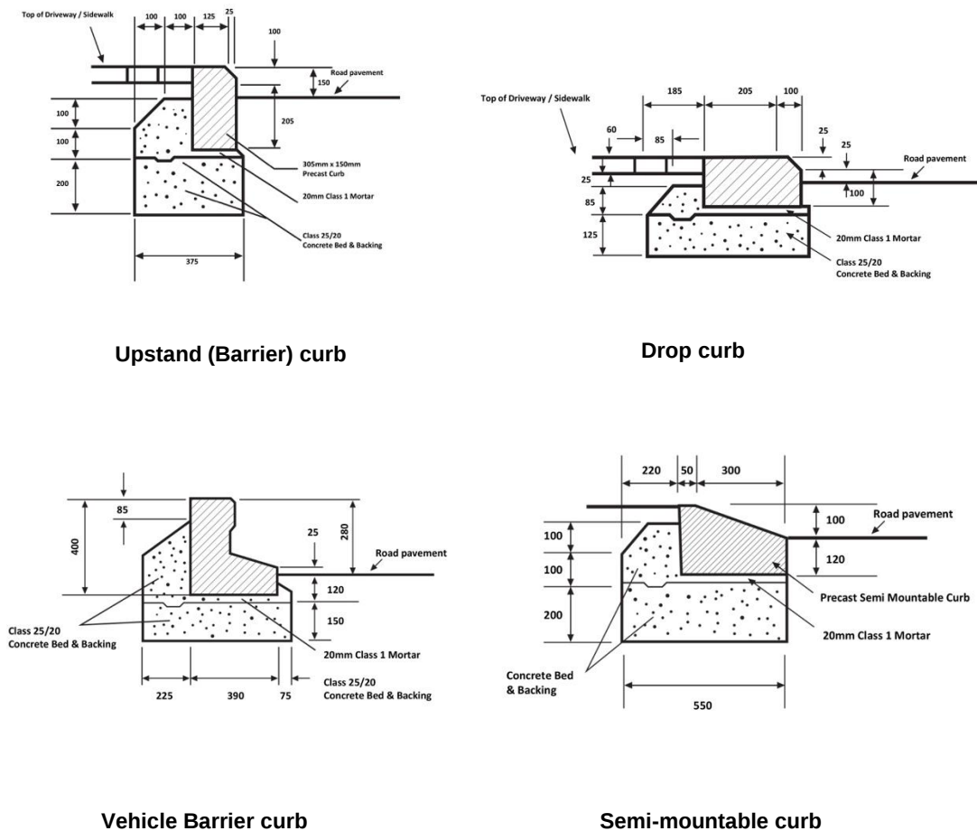
Figure 10 Curb Profiles
