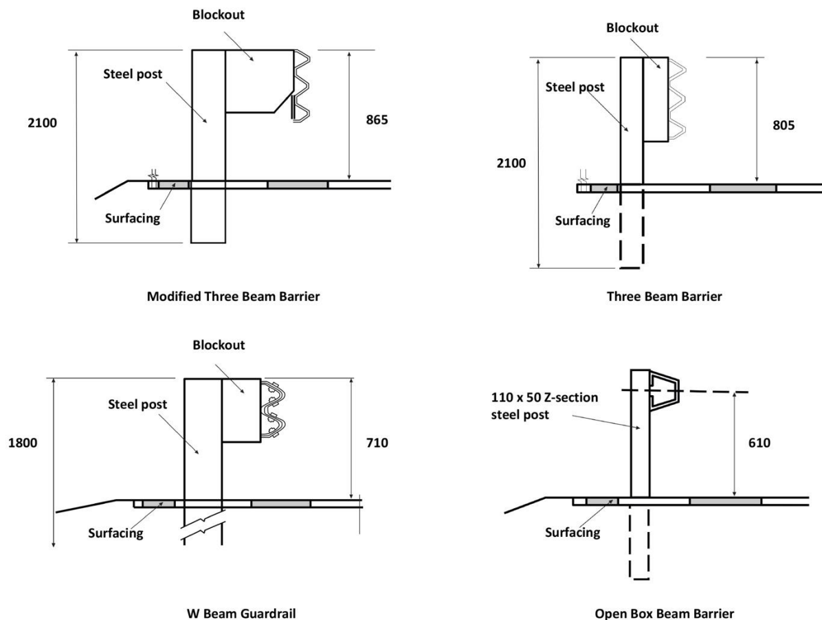
Figure 6 Profiles of Four Common Types of Semi-rigid Barriers
